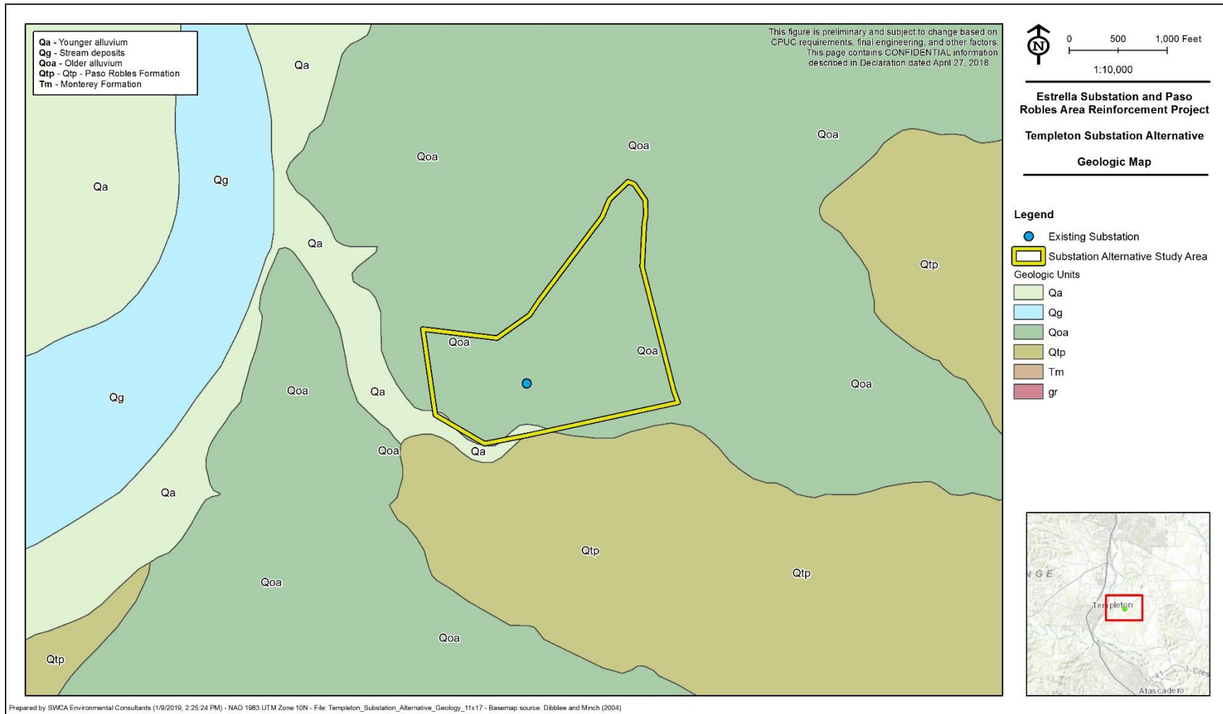
Figure 3. Geologic Map
